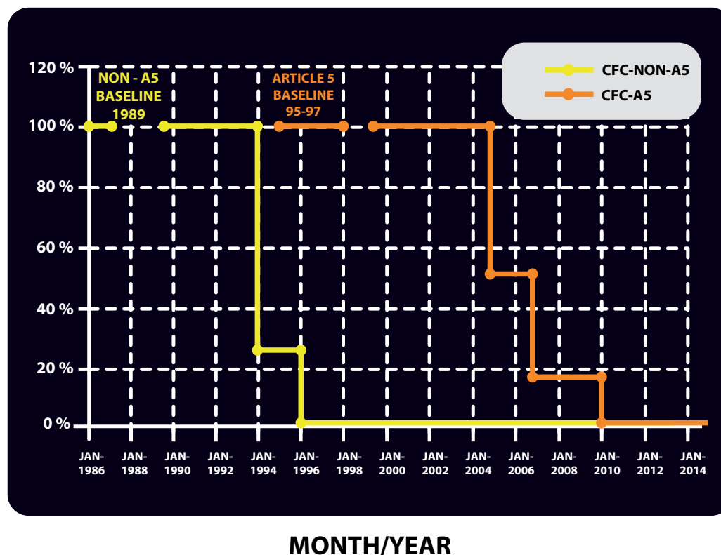
Figure 1.3 Article 5 and Non-Article 5 countries phase-out schedules of Annex A Group I CFCs
