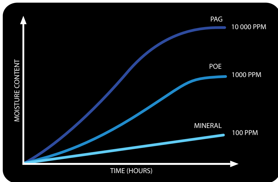
Hygroscopy of POE and mineral lubricants
