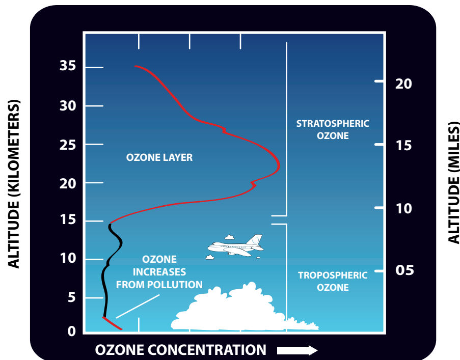
Distribution of ozone in atmosphere.
