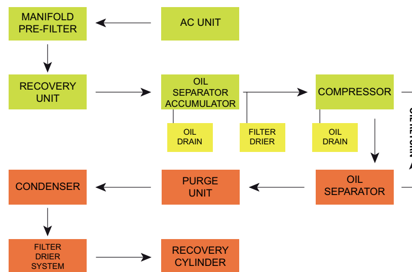
Typical single pass system
