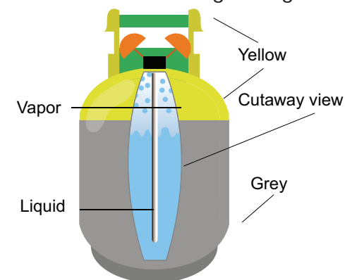
Cylinder with separate liquid and gas valves
