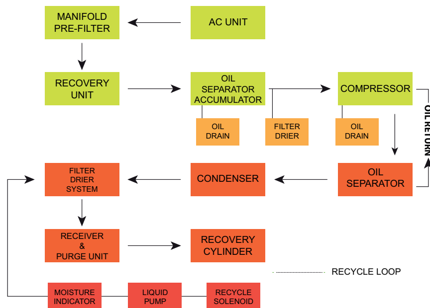
Typical multi-pass system
